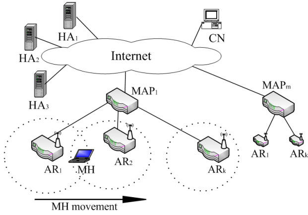
Fig. 1. HMIPv6 Architecture.
