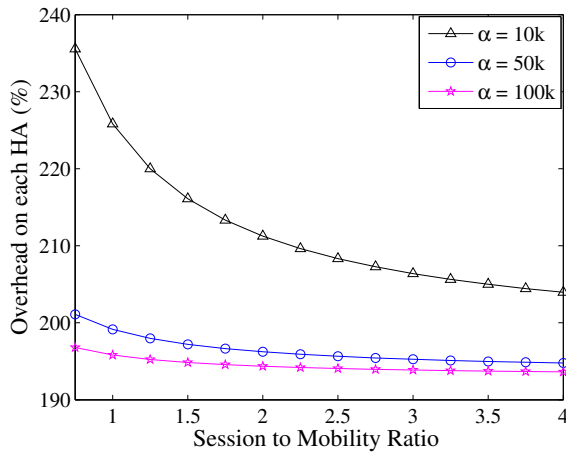
Fig. 4. Percentage overhead on each HA vs. session to mobility ratio for different session size.
